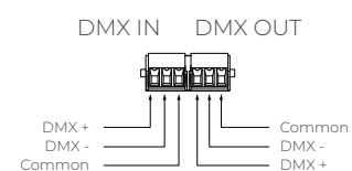
Phoenix Connector
